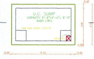
SUMP DETAIL SCALE 1"=4'-0"
