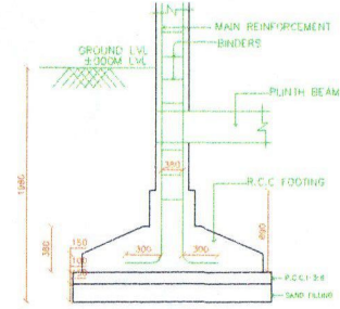
TYPICAL SECTION OF R.C.C. COLUMN FOUNDATION SCALE 1"=2'-0"
