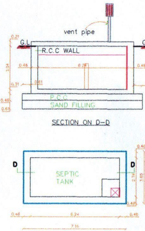
PLAN OF SEPTIC TANK SCALE 1"=2'-0"
