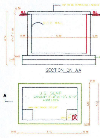
SUMP DETAIL SCALE 1"=4'-0"
