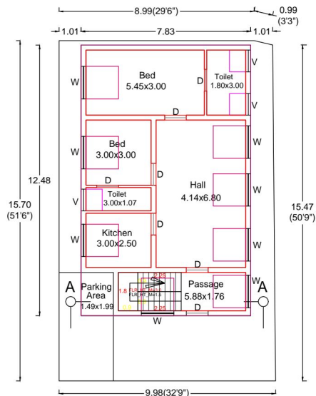
PLAN - G.F (Facing EAST)
