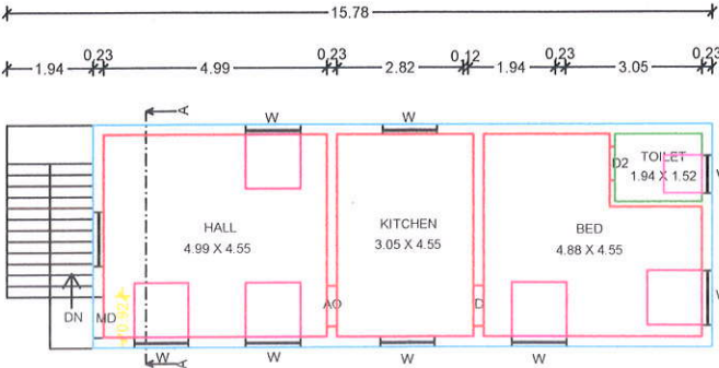
PRO. FIRST FLOOR PLAN
