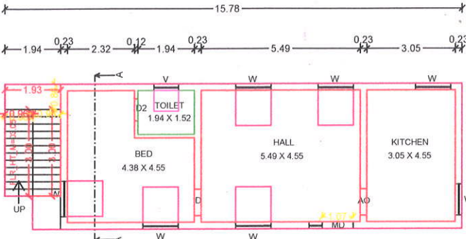
PRO. GROUND FLOOR PLAN
