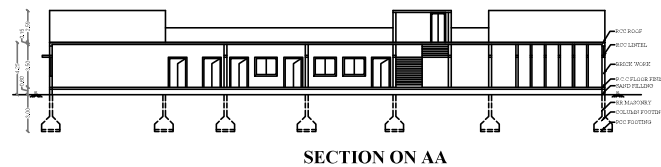
SECTION ON AA
