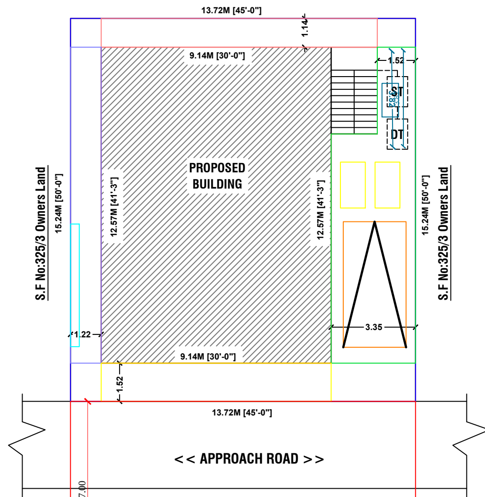
SITE PLAN
