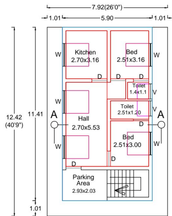
PLAN - G.F ( Facing NORTH)
