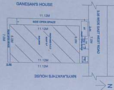
PERIYA THAMARIS HOUSE SITE PLAN SCALE - 1:100
