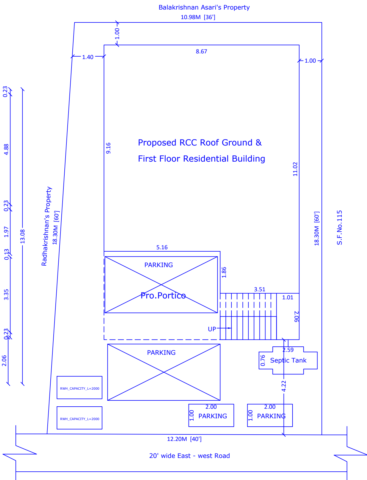
SITE PLAN
