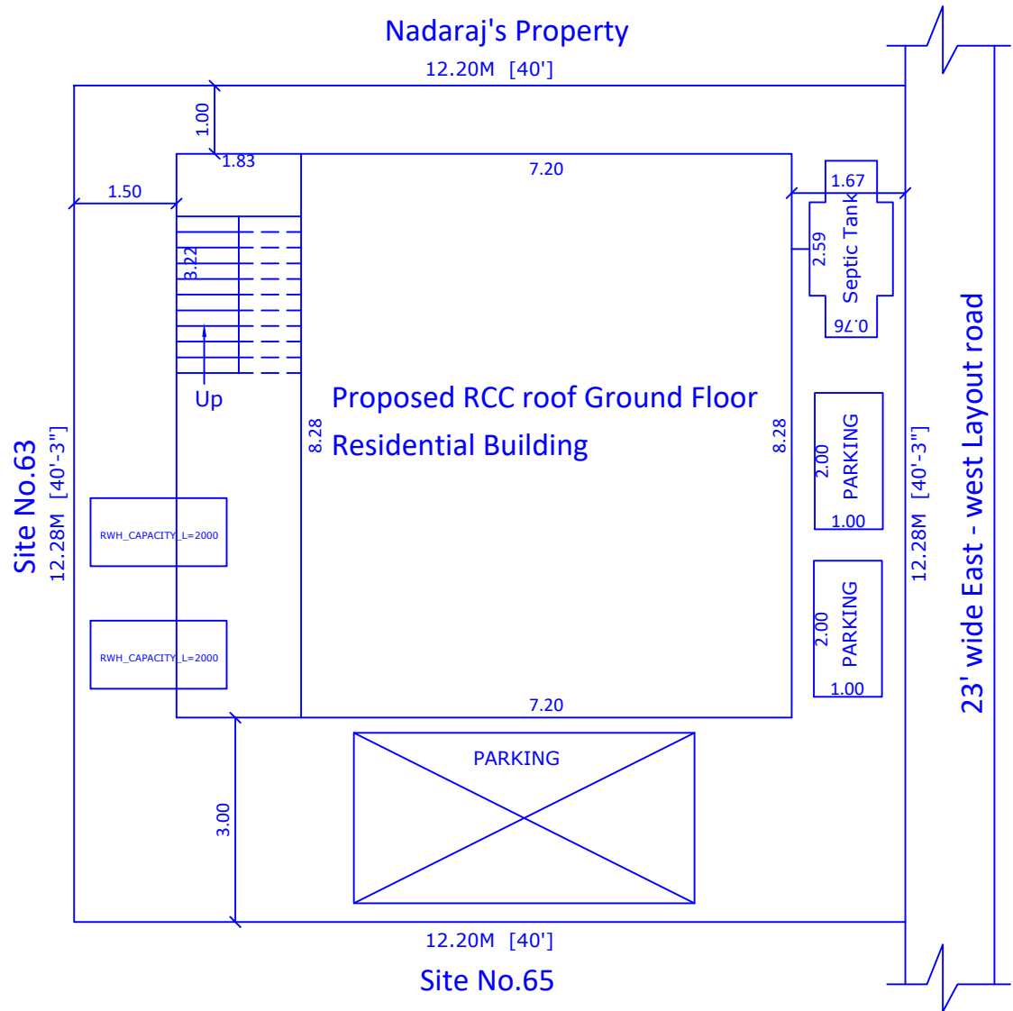
SITE PLAN
