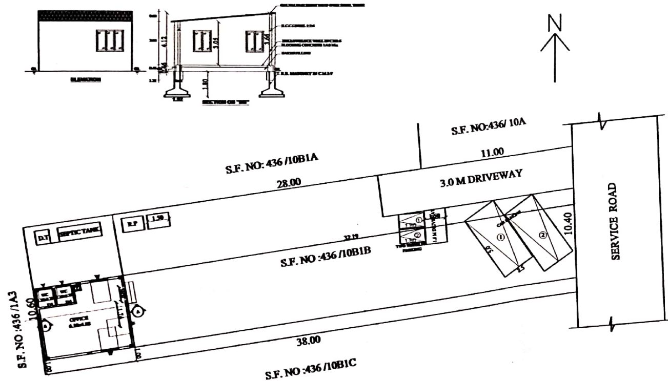
SITE CUM GROUND FLOOR PLAN
