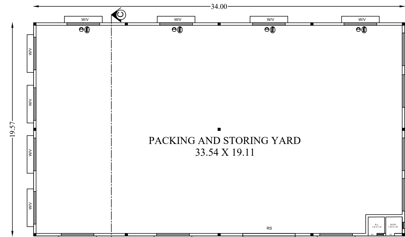
PLAN - BLOCK - 3
