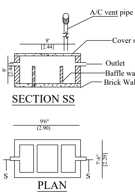
PLAN - BLOCK - 1
