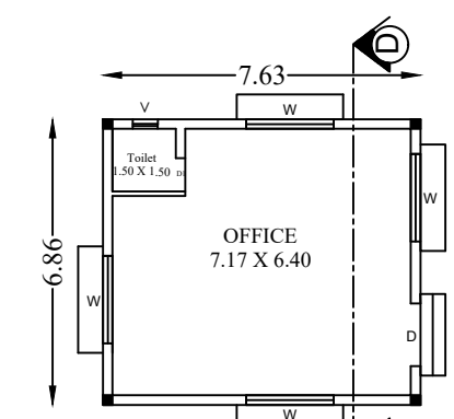
PLAN - BLOCK - 4
