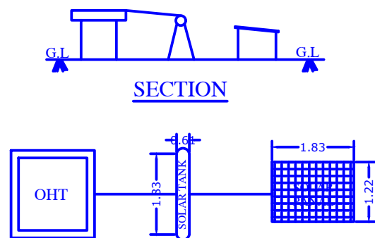
SOLAR SYSTEM PLAN
