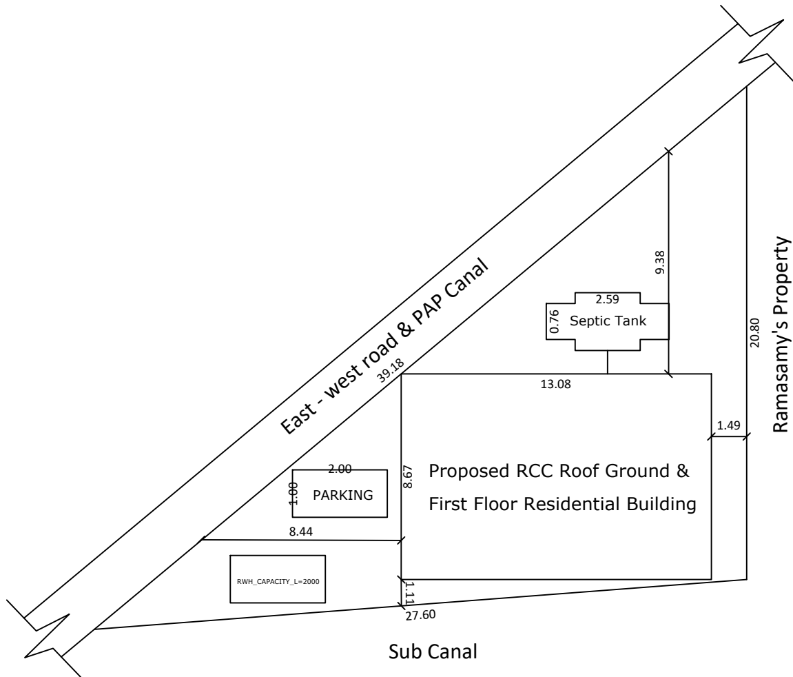
SITE PLAN
