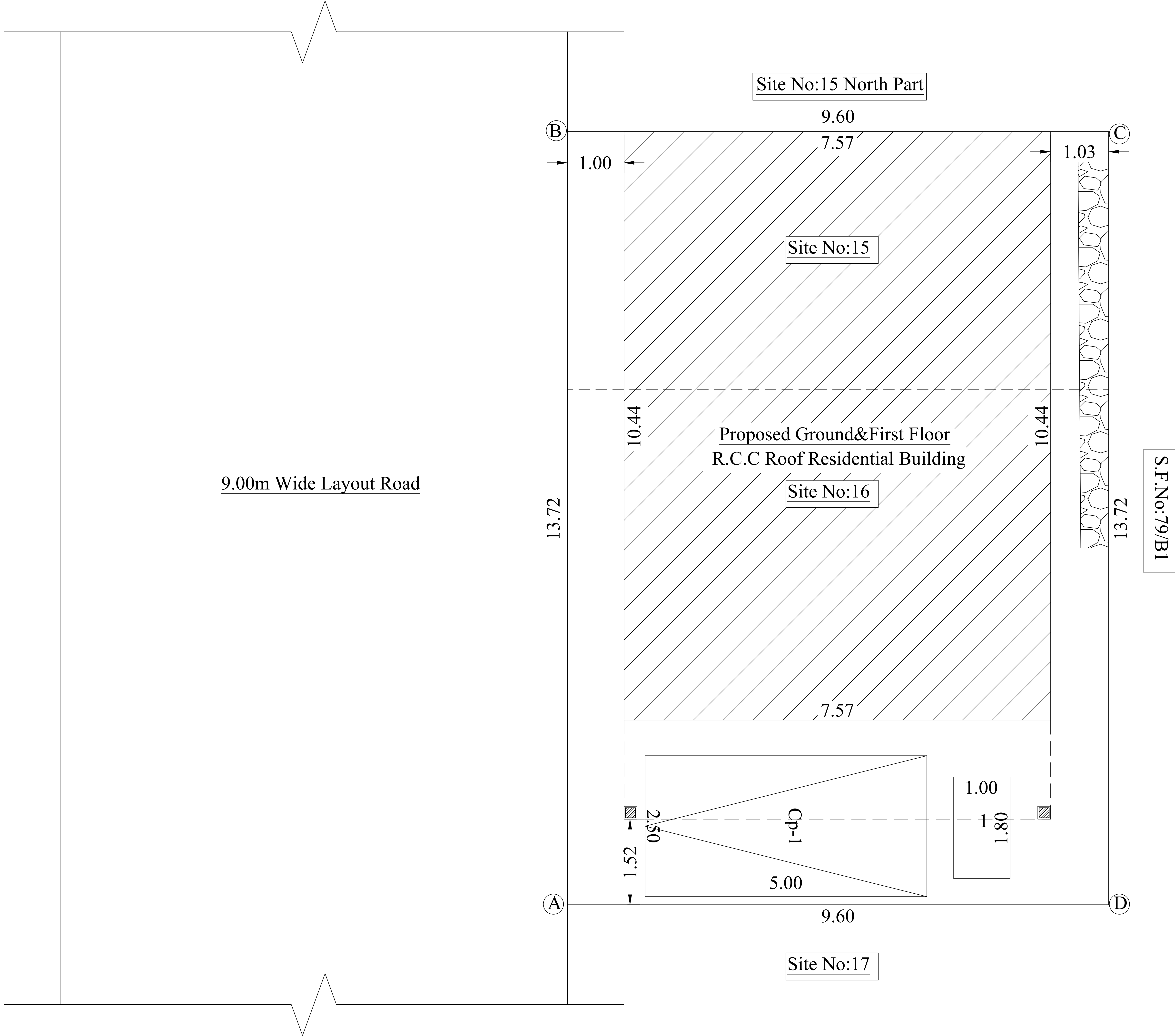
Site Plan
