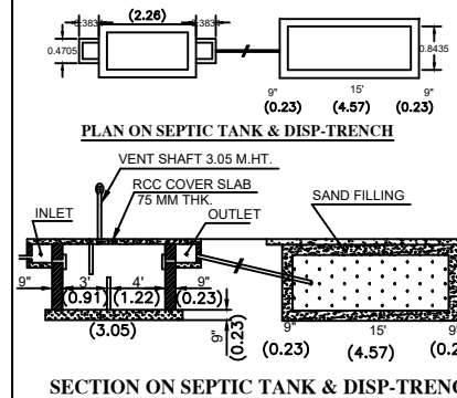
SECTION ON SEPTIC TANK & DISP-TRENCH
