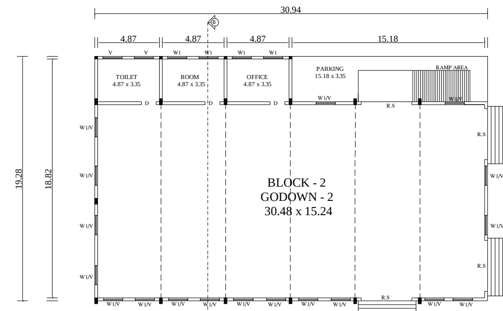
BLOCK - 2 - GROUND FLOOR PLAN
