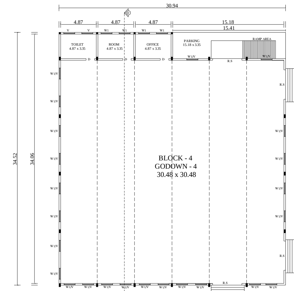
BLOCK - 4 - GROUND FLOOR PLAN
