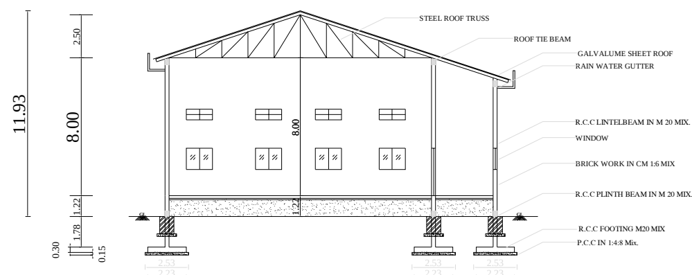
SECTION ON C-C
