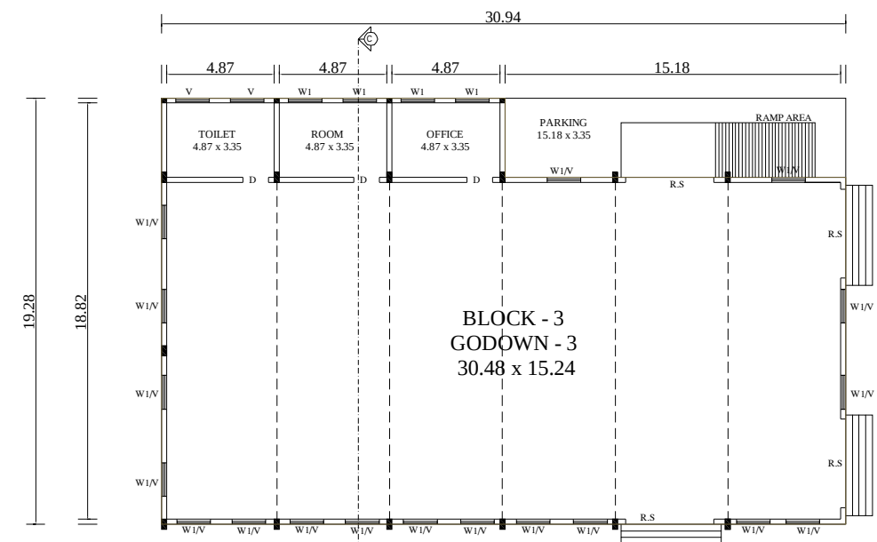
BLOCK - 3 - GROUND FLOOR PLAN
