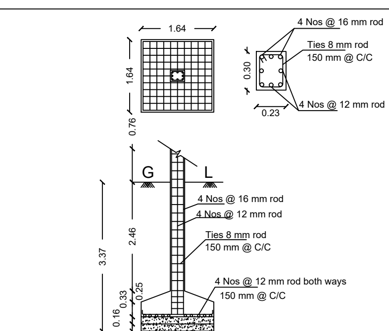
COLUMN AND FOOTING DETAILS
