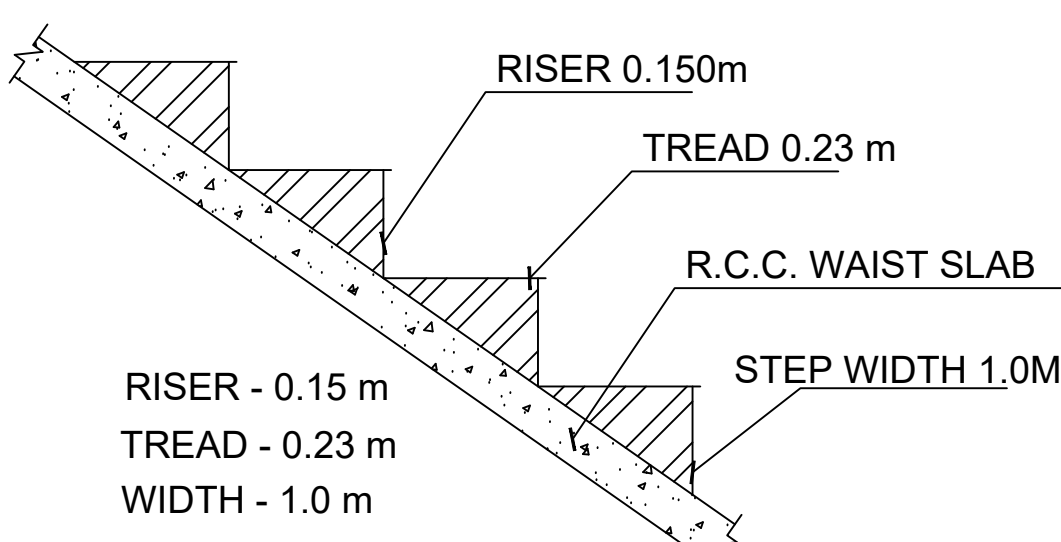
STAIRCASE DETAILS
