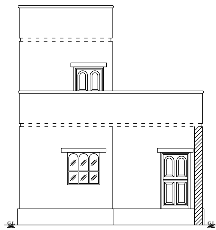
ELEVATION (Facing on South)
