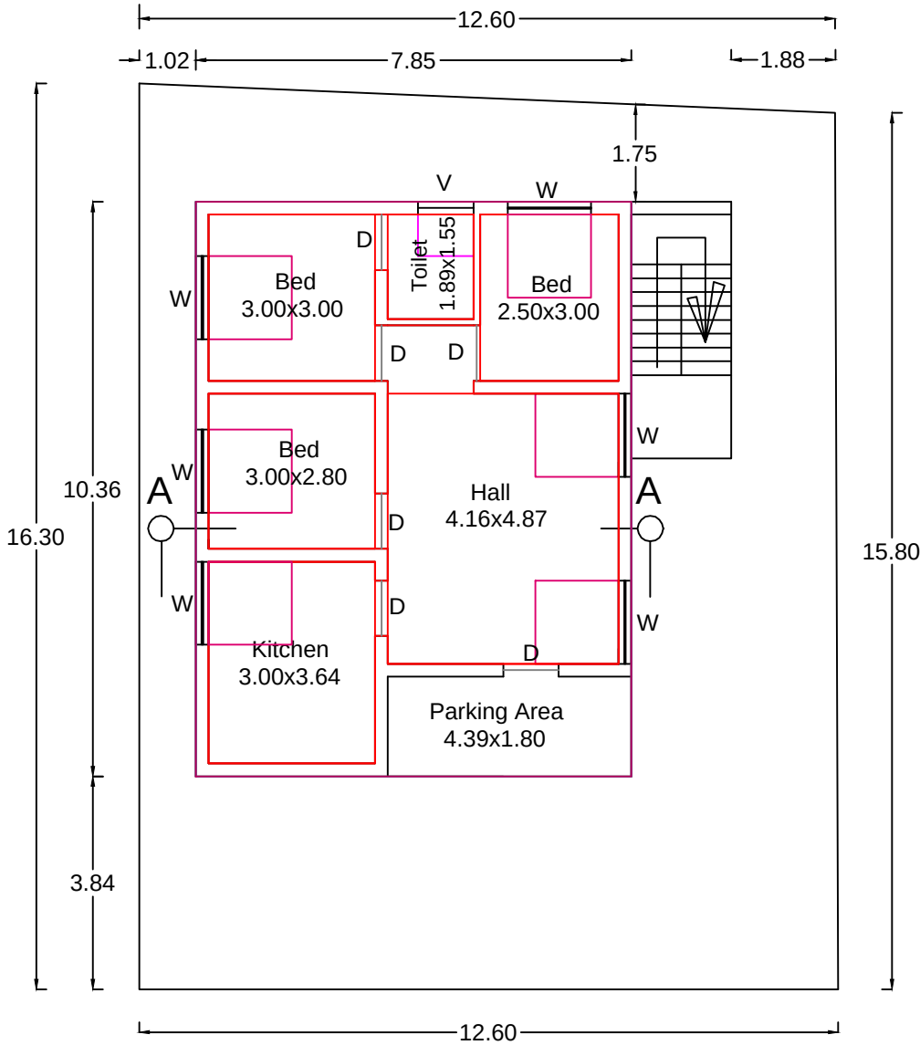
PLAN - G.F ( Facing EAST)
