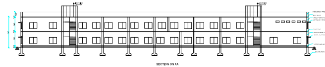
SECTION ON AA
