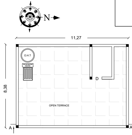
SECOND FLOOR PLAN FACING EAST
