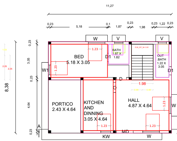
GROUND FLOOR PLAN FACING EAST
