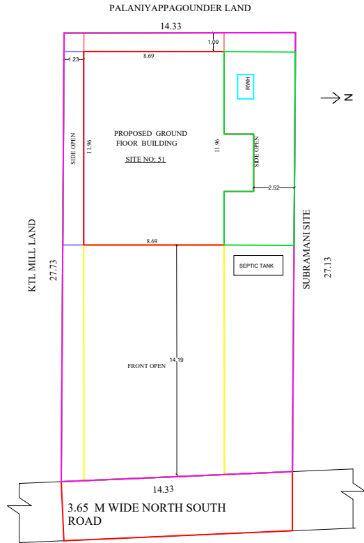
SITE PLAN
