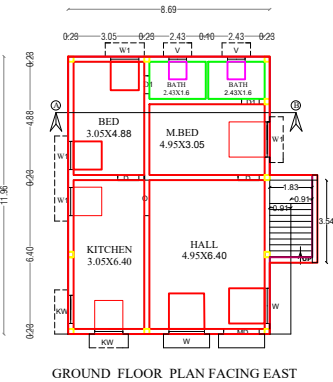
GROUND FLOOR PLAN FACING EAST
