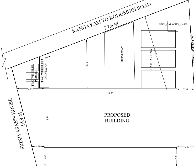
SITE PLAN
