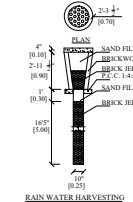
RAIN WATER HARVESTING PERCOLATION PIT
