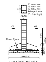
COLUMN DETAILS
