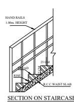
SECTION ON STAIRCASE
