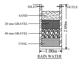
RAIN WATER COLLECTION TANK
