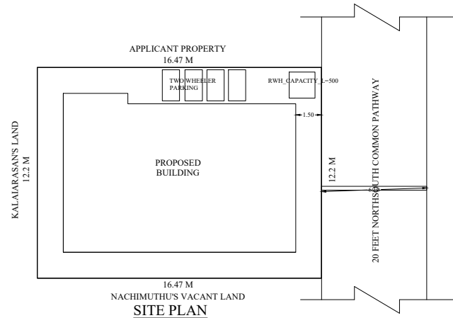
SITE PLAN
