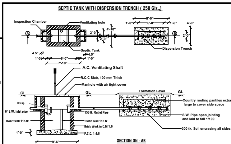
Rain Water Perculation Pit (Not to Scale)
