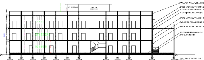
SECTION ON "X-Y"
