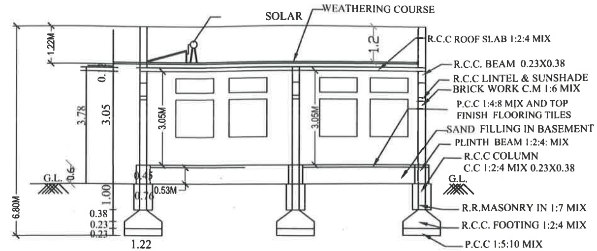
SECTION PLAN
