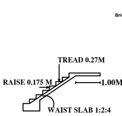
STAIRCASE DETAILS
