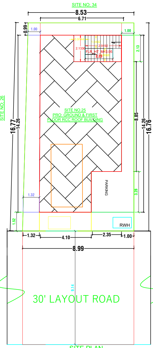
SITE PLAN
