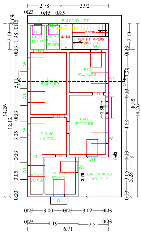
GROUND FLOOR PLAN FACING EAST
