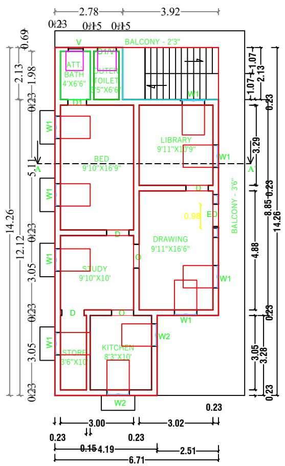
FIRST FLOOR PLAN FACING EAST
