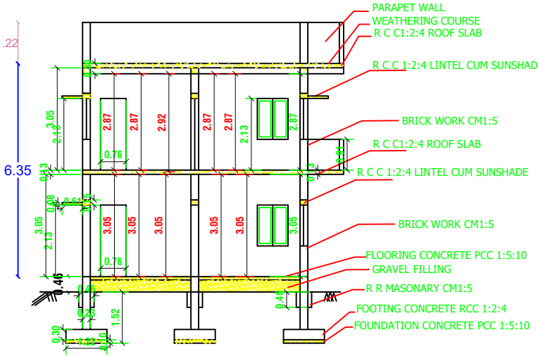
SECTION-AA&A'
