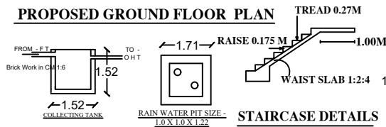
STAIRCASE DETAILS
