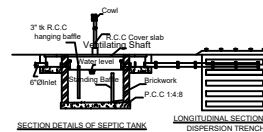
SECTION DETAILS OF SEPTIC TANK
