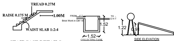
STAIRCASE DETAILS
