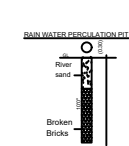
RAIN WATER PITS DETAIL (NTS)
