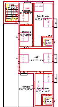
EXISTING GROUND FLOOR PLAN
