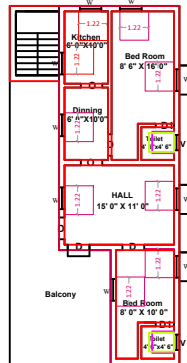
PROPOSED FIRST FLOOR PLAN
