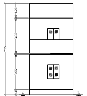
ELEVATION FACING EAST
