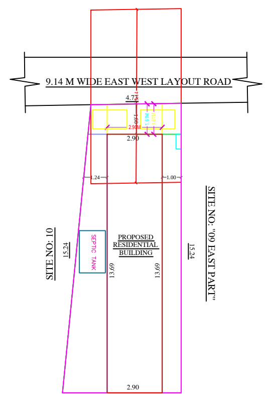
S.P.RAJU & SUNDARAM PROPERTY SITE PLAN 1:100
