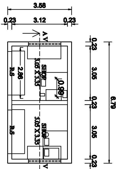
DETAILED PLAN
