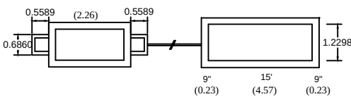
PLAN ON SEPTIC TANK & DISP-TRENCH
