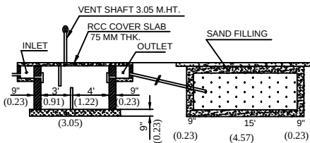
SECTION ON SEPTIC TANK & DISP-TRENCH
