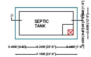
PLAN OF SEPTIC TANK SCALE 1"=2'0"
