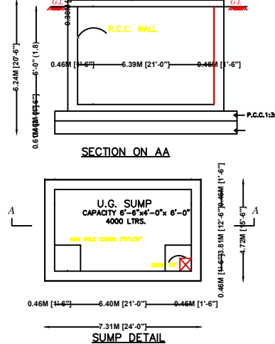
SUMP DETAIL SCALE 1"=4'0"
