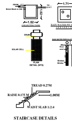
STAIRCASE DETAILS
