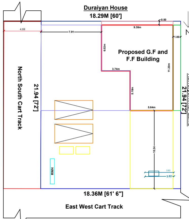
SITE PLAN
