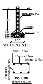
SECTION ON CC
