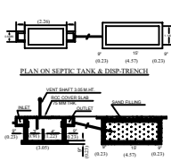
SECTION ON SEPTIC TANK & DISPOSAL TRENCH
