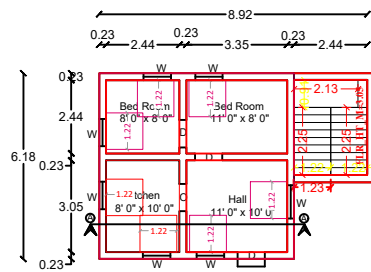
EXISTING GROUND FLOOR PLAN
