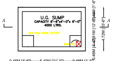
SUMP DETAIL SCALE 1"=4'-0"
