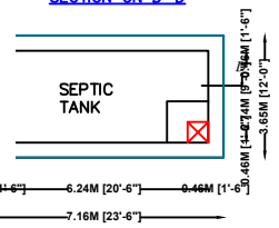
PLAN OF SEPTIC TANK SCALE 1"=2'0"
