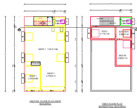
FIRST FLOOR PLAN (RESIDENTIAL BUILDING)
