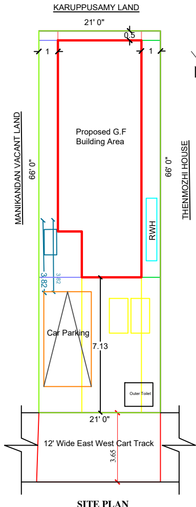
SITE PLAN
