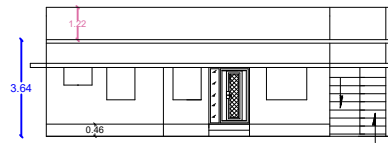
ELEVATION (FACING EAST)
