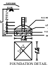
FOUNDATION DETAIL
