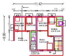
FLOOR FACING EAST
