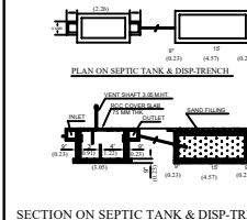
SECTION ON SEPTIC TANK & DISP-TRENCH
