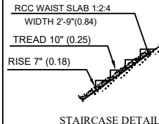
STAIRCASE DETAIL
