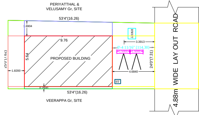
SITE PLAN SCALE 1: 100
