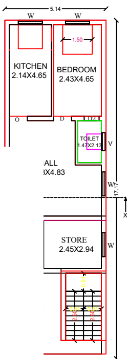
1D FLOOR PLAN
