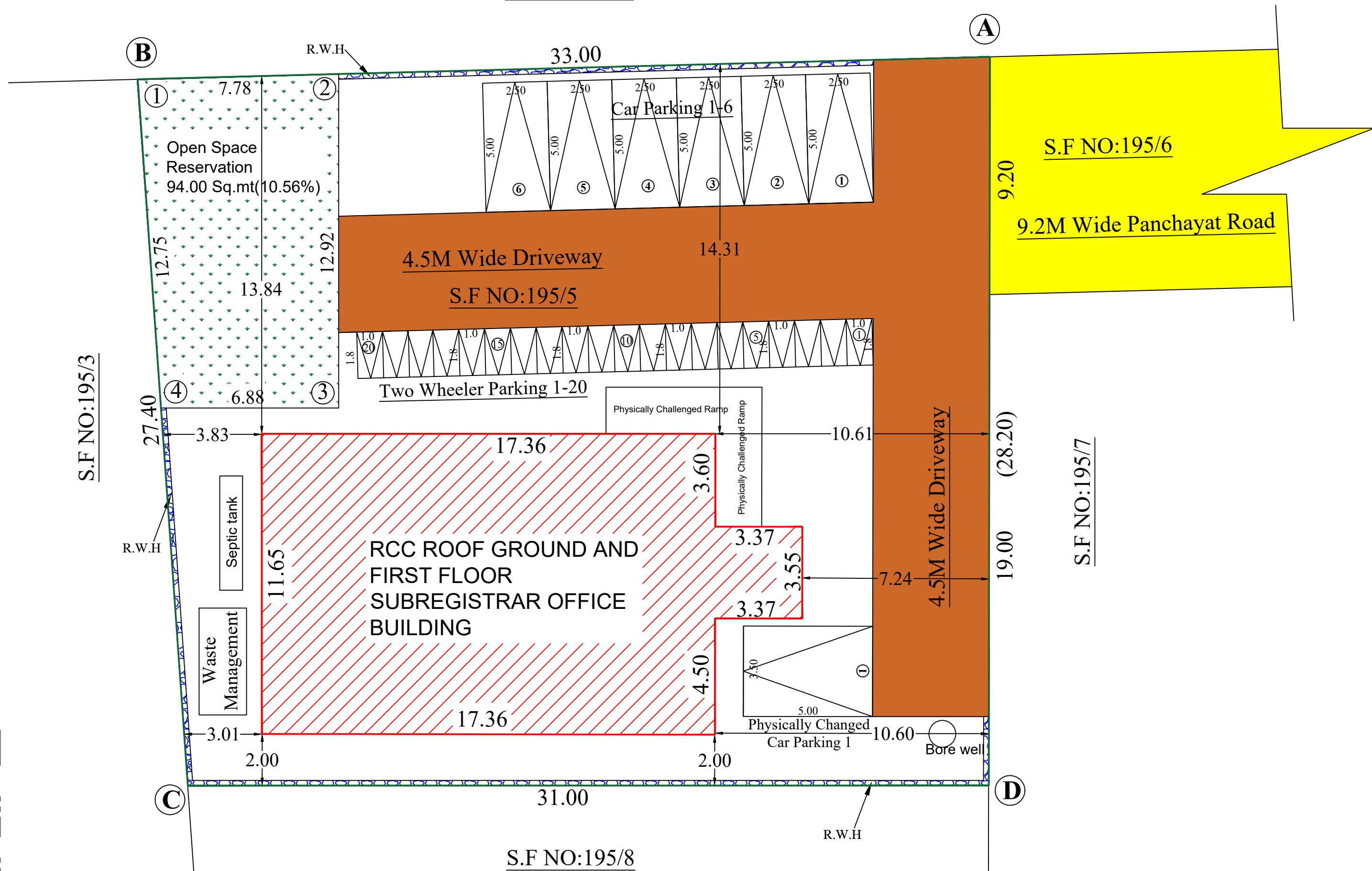
SITE PLAN (1:100)
