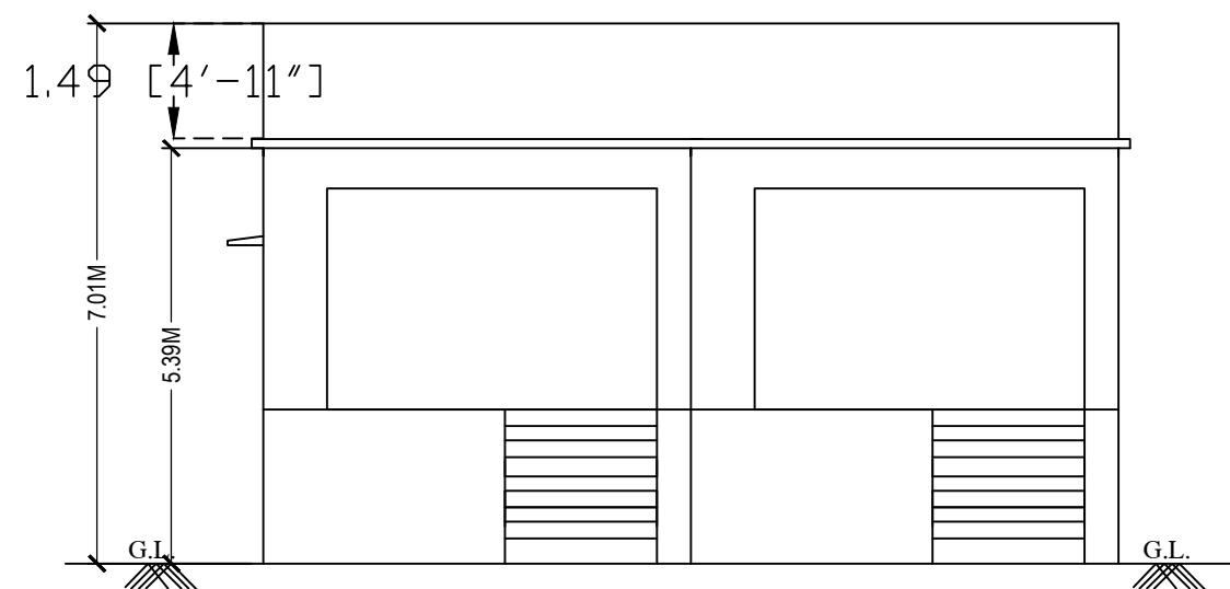
WEST ELEVATION
