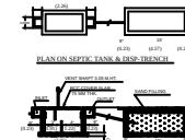
SECTION ON SEPTIC TANK & DISP-TRENCH
