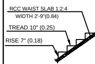
STAIRCASE DETAIL
